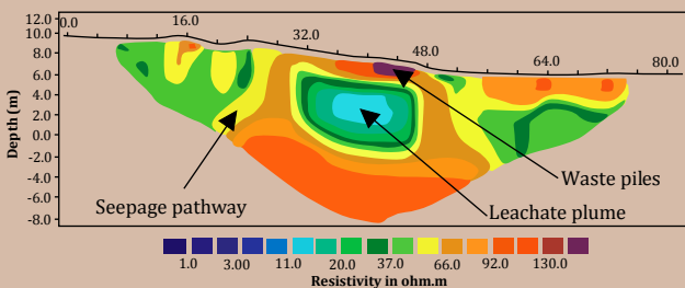
A 2D resistivity profile of a landfill site
